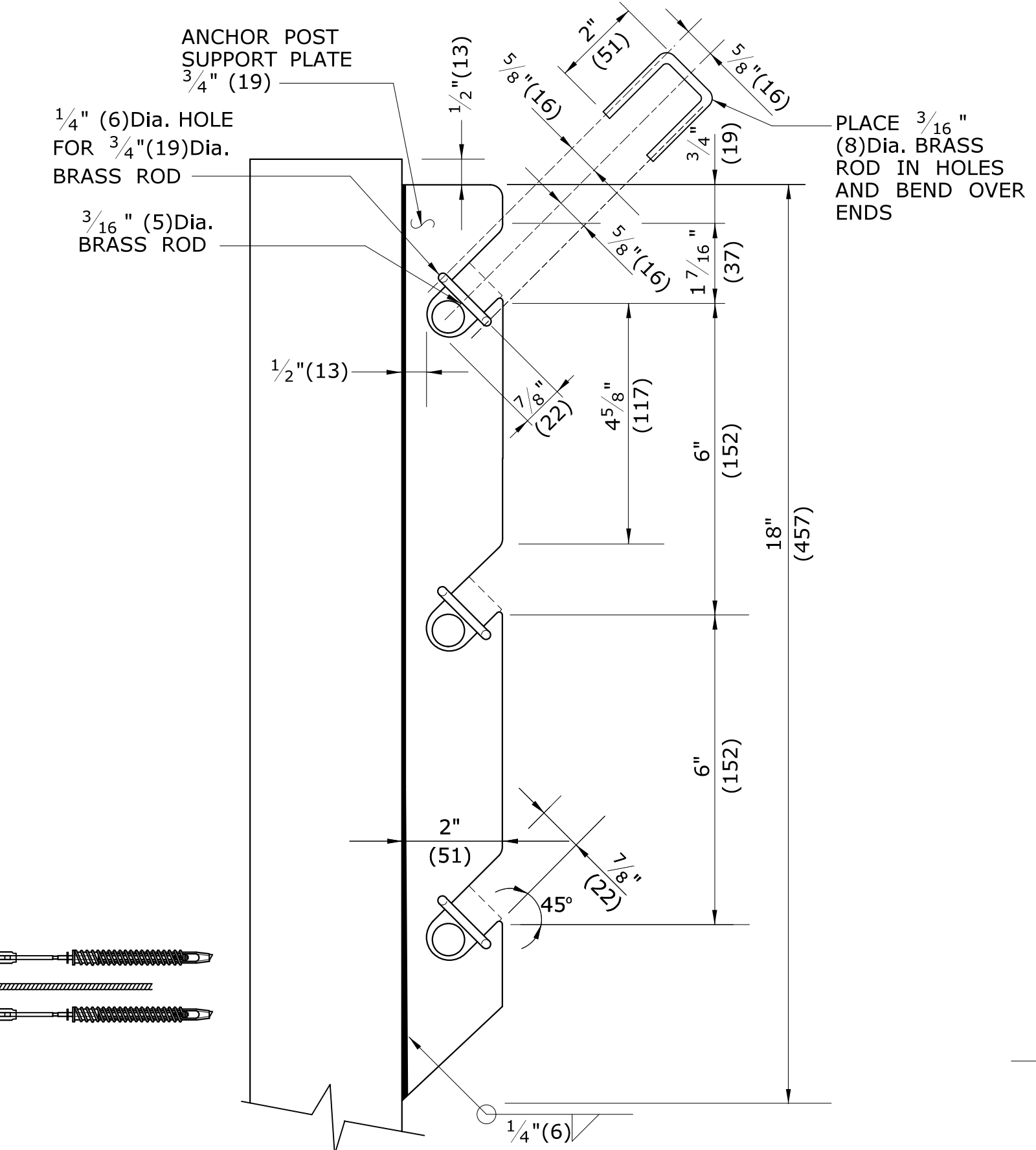
SIDE VIEW OF UPPER ANCHOR POST AT TOP
