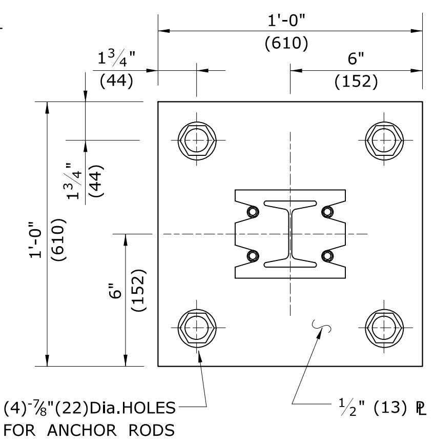
ANCHOR POST AND BASE PLATE
