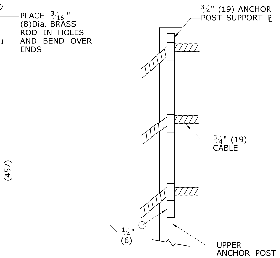
FRONT VIEW OF POST TOP (ROAD SIDE)
