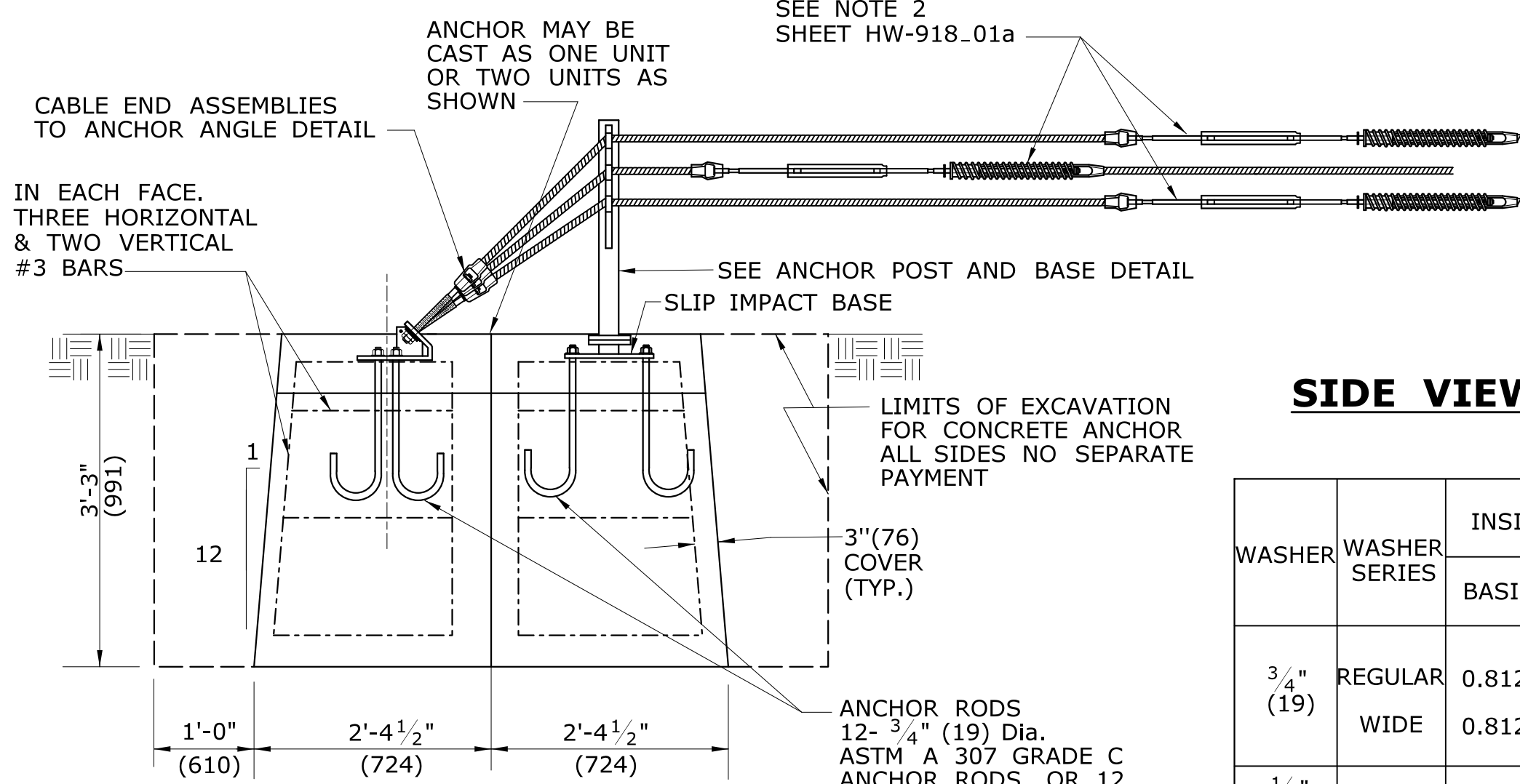
SECTION A ANCHOR UNIT WITH REINFORCEMENT (TWO PIECE) LEFT HAND
