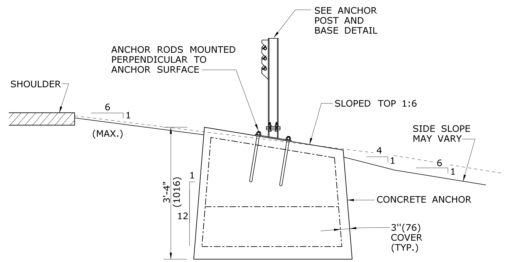
SECTION B OFFSET AND GRADES FOR INSTALLATION (LEFT HAND)
