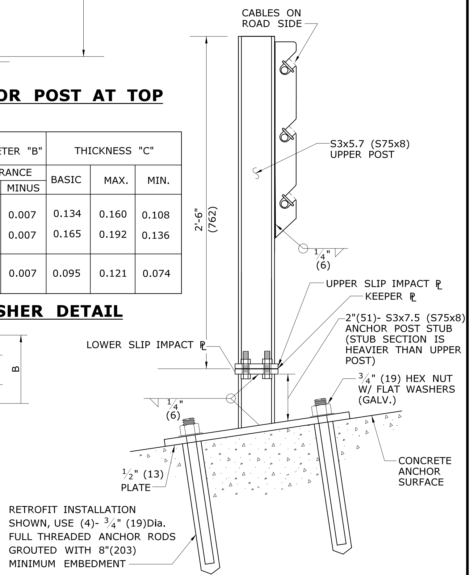
ANCHOR POST AND BASE DETAIL NOTE: SEE THE ANCHOR UNIT DETAIL FOR TYPICAL INSTALLATION
