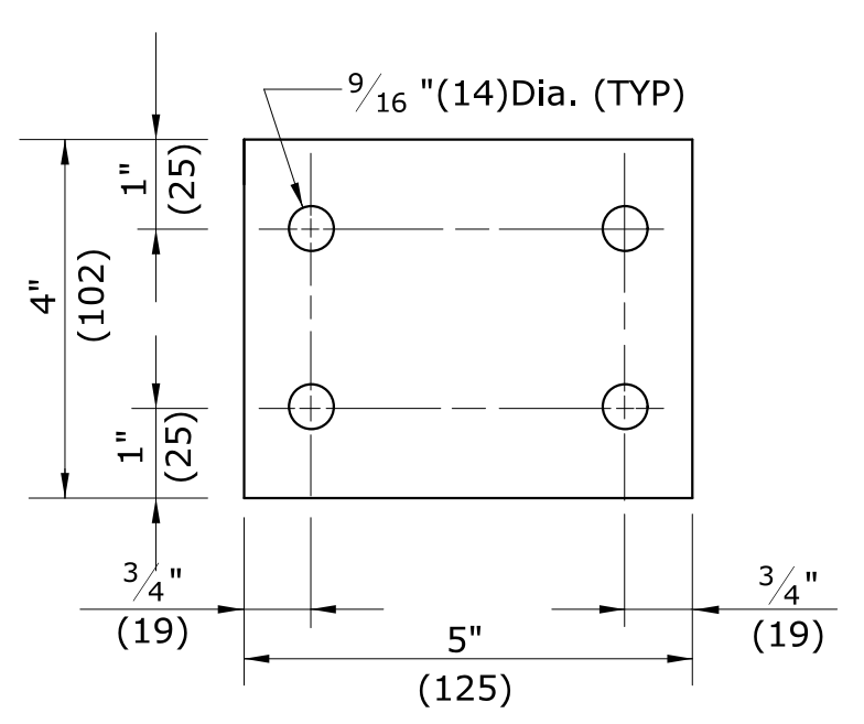
KEEPER PLATE (28 GA. GALV. STEEL, PAINTED ORANGE)
