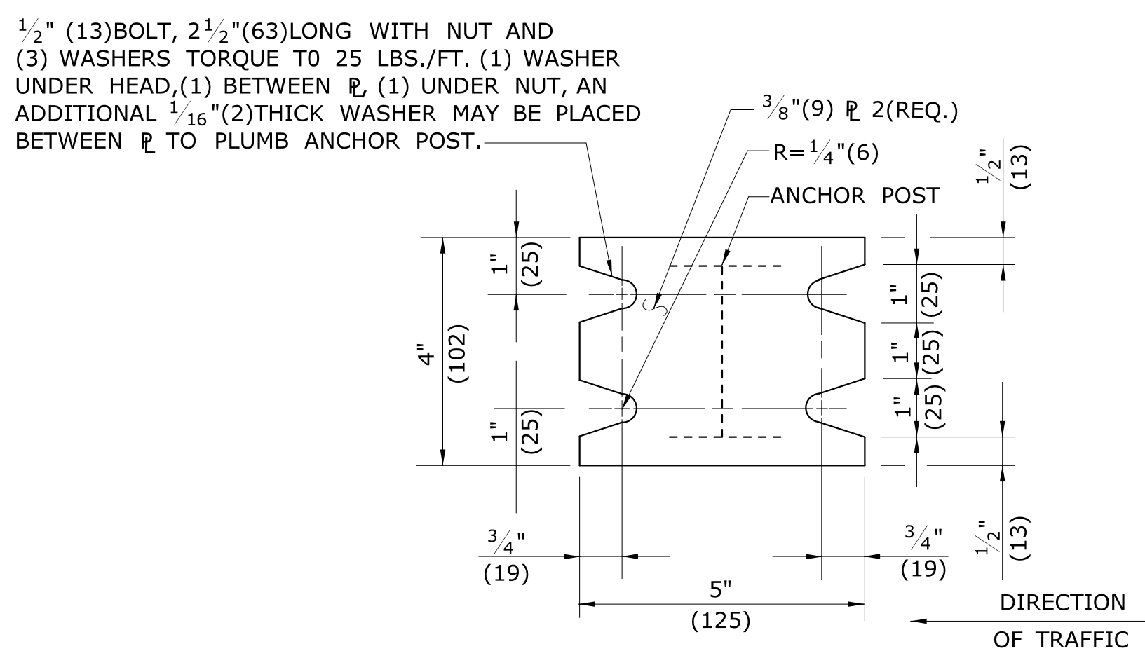
SLIP IMPACT BASE (KEEPER PLATE NOT SHOWN)
