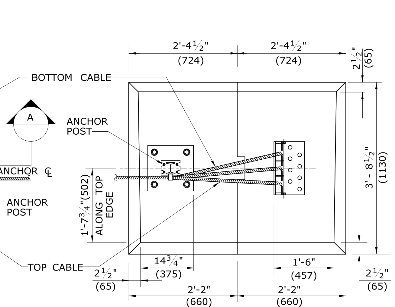
ANCHOR UNIT TOP VIEW RIGHT HAND
